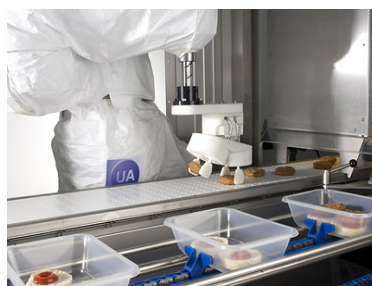
Scara-Roboter greift Fleisch-Patties / scara robot handling meat patties
