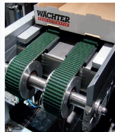
Zuführung der Wellpappentrays / feeding of the corrugated trays
